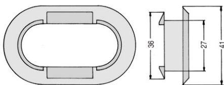
Handhold protector
