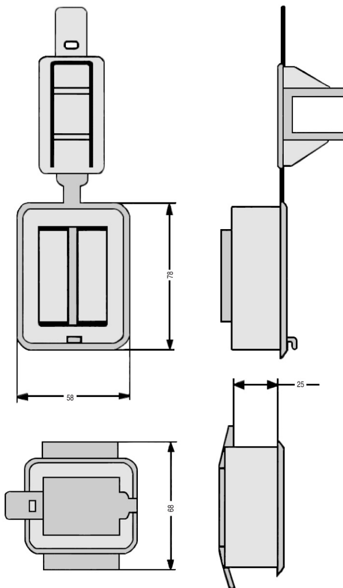
EKS 892.0 Large locking device
