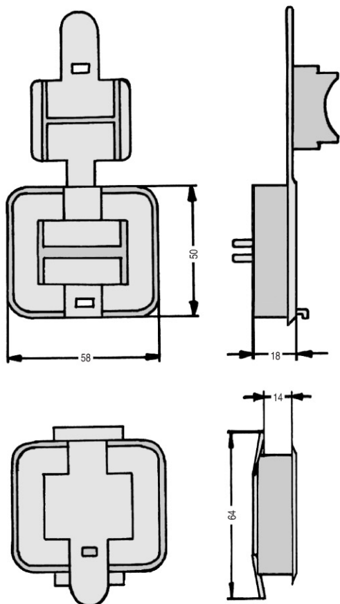
EKS 891.0 Small locking device
